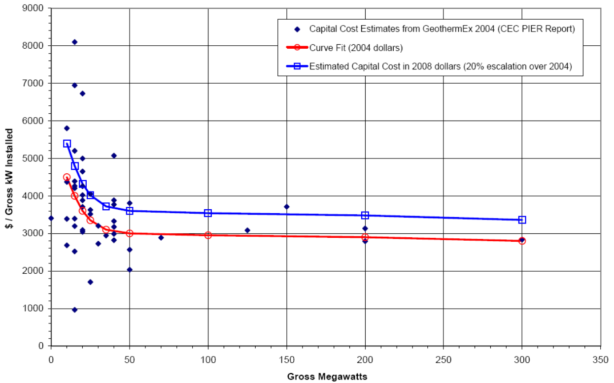
Figure 2: Geothermal capital cost estimates for RETI study
