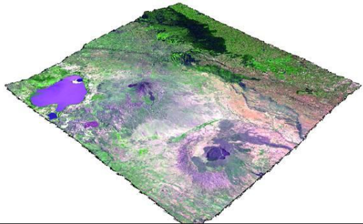
Figure 49: 3D view of Olkaria volcano Digital Elevation Model (Baseheights are obtained from ASTER DEM)
