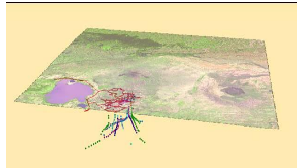
Figure 8 b: 3D view of the geothermal directional wells, road network in a LANDSAT image. The base heights were from ASTER DEM shown in Figure 6.
