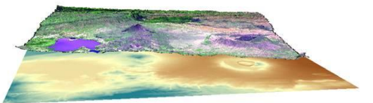
Figure 51: LANDSAT Image draped on an ASTER DEM for Olkaria Volcano
