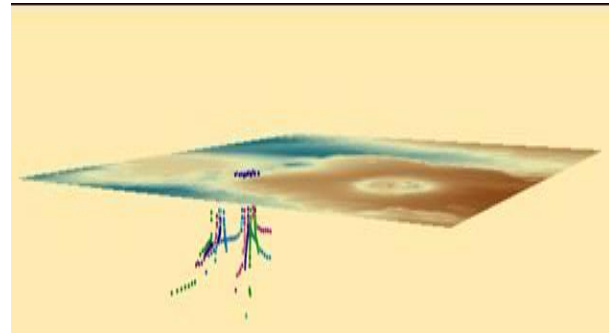
Figure 52a: ASTER DEM model of Olkaria geothermal field showing 3D view of geothermal directional wells.
