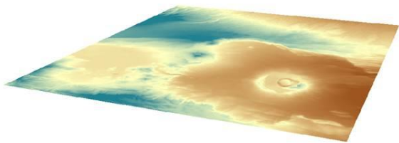
Figure 50: An ASTER DEM that is registered in GIS.
