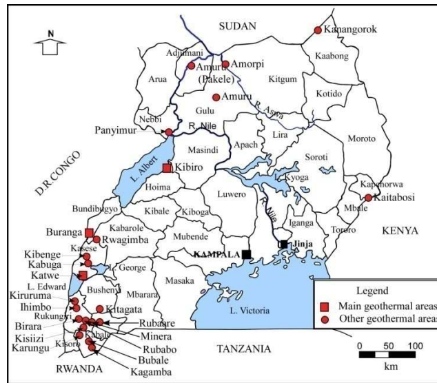
Figure 1: The geothermal areas of Uganda.
