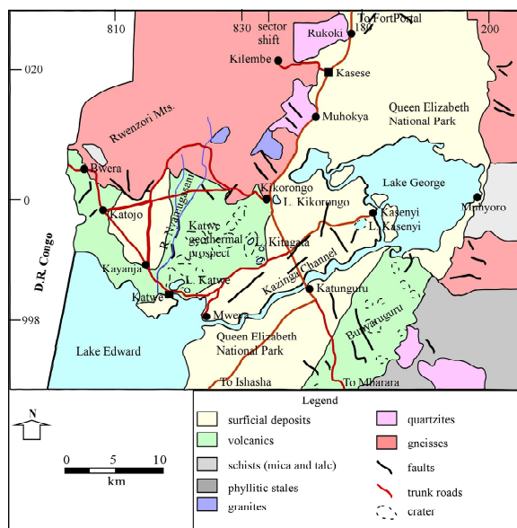
Figure 2: Geology of Katwe volcanic field and surroundings.
