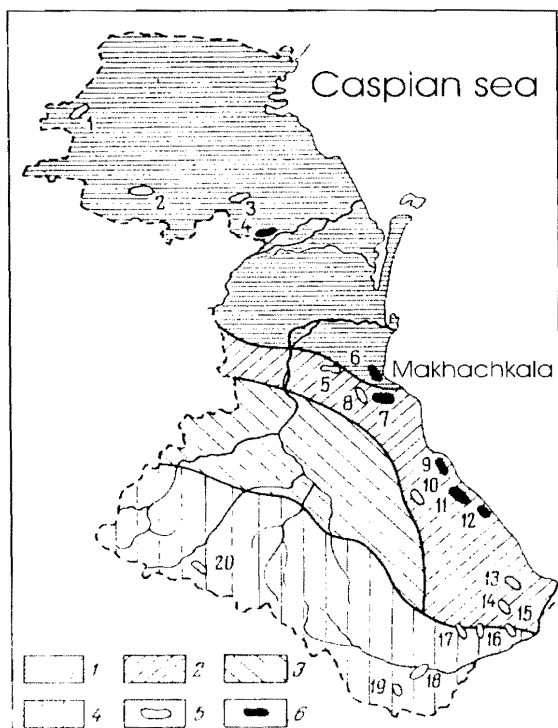
Figure 2. Map of hydrogeothermal deposits and perspective areas of Dagestan
