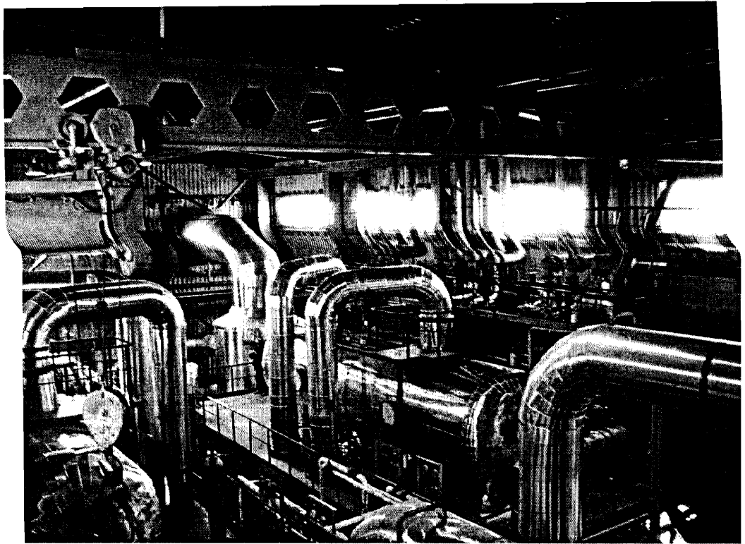
Figure 4,b. Mutnovsky geothermal power plant (MGeoPP). Primary separators provide MGeoPP with the high-quality steam. Photo of Svalova V.B.
